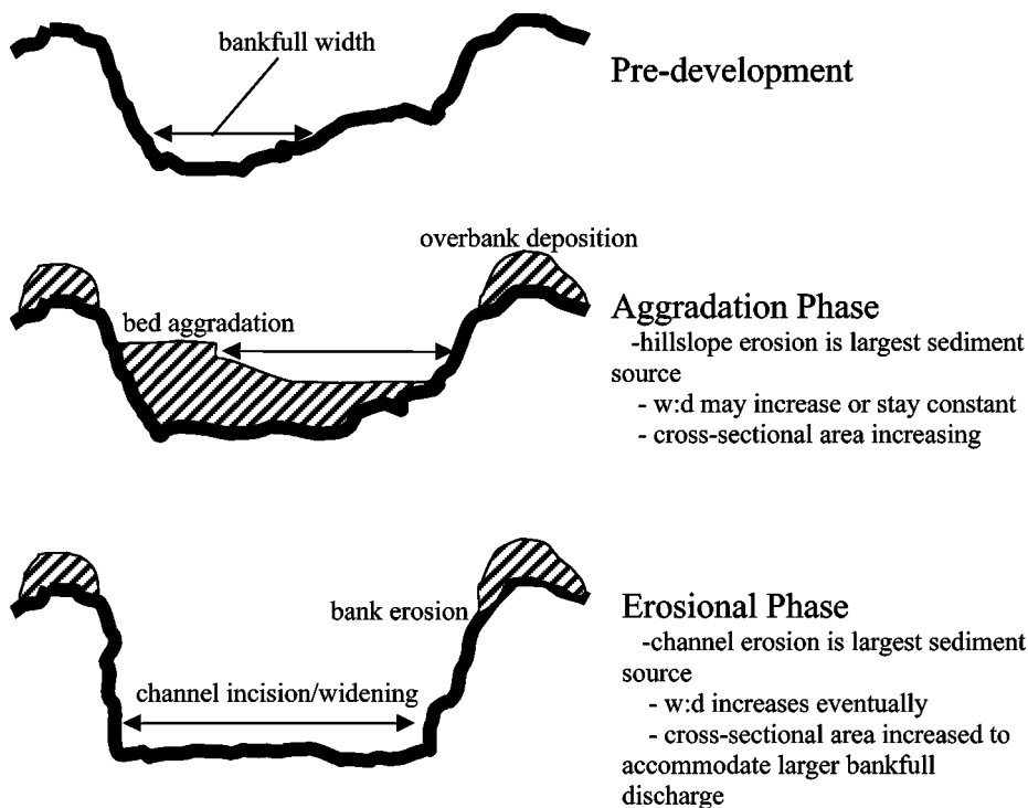
Figure 2 Channel changes associated with urbanization. During the construction phase of urbanization, hillslope erosion increases sediment supply leading to bed aggradation and overbank deposition. After construction ceases hillslope sediment supply is reduced, but bankfull flows are increased owing to increases in imperviousness. This leads to increased channel erosion as channel incision and widening occur to accommodate increased bankfull discharge.
