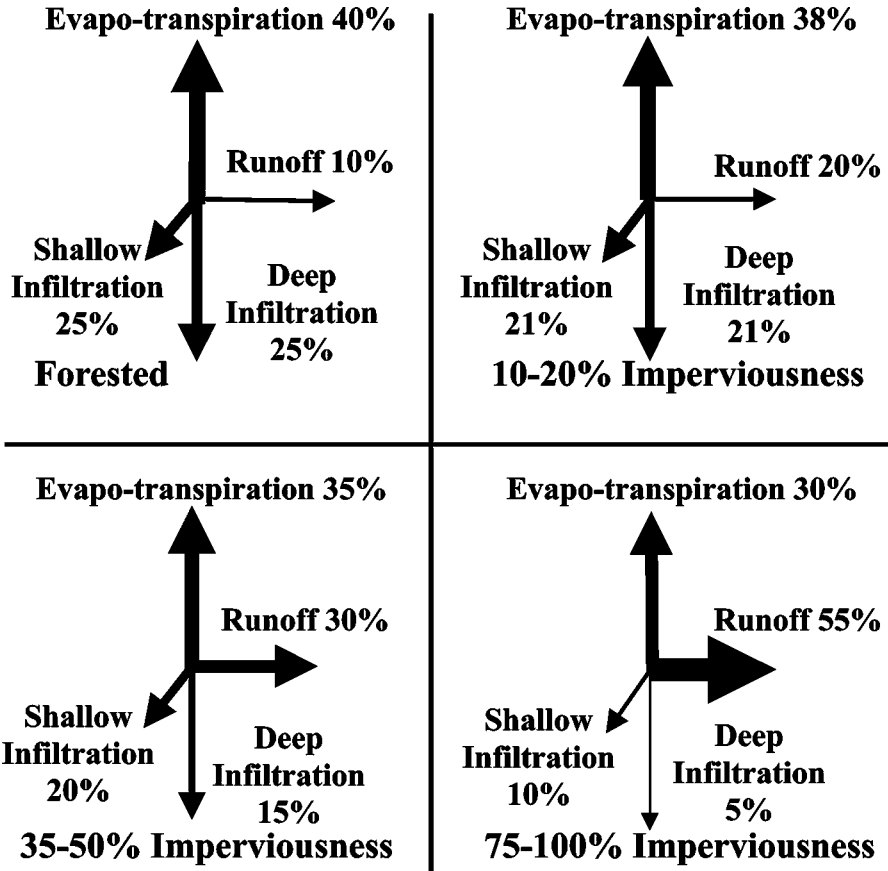
Figure 1 Changes in hydrologic flows with increasing impervious surface cover in urbanizing catchments (after Arnold & Gibbons 1996).
